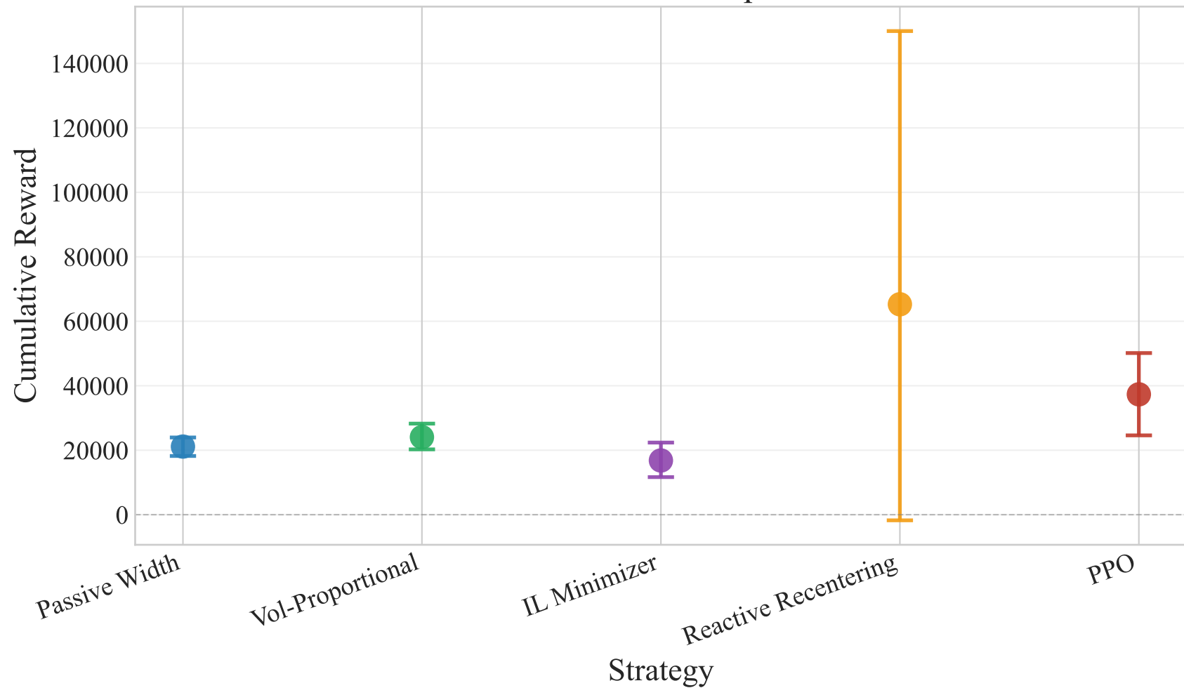
Mean Rewards with 95% Bootstrap Confidence Intervals
