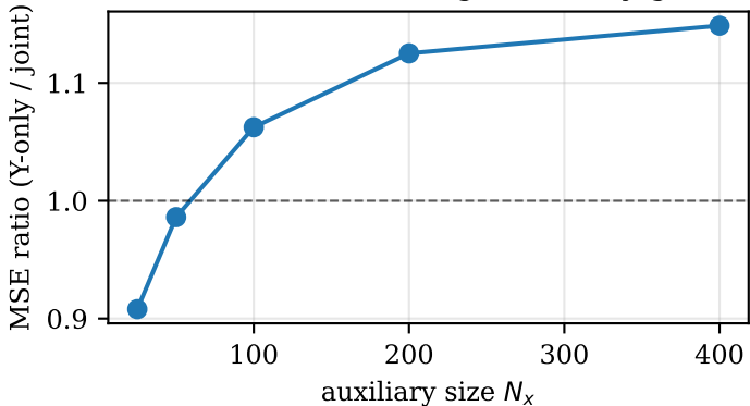
E3: transfer-learning efficiency gain
