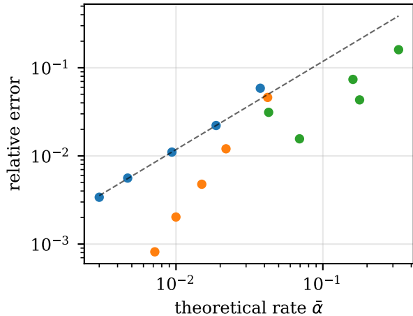
(b) loadings \Lambda
