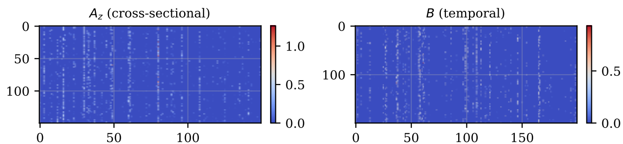
Figure 5: Learned, frozen A_z ( N \times N ) and B ( T \times T ) from the independent-sample linear model.
