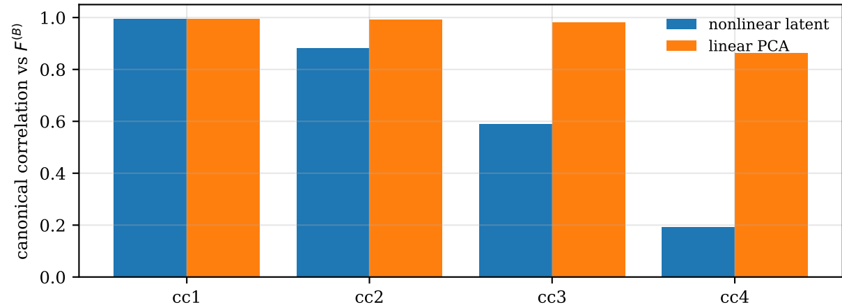
E4: factor-space recovery on linear truth
