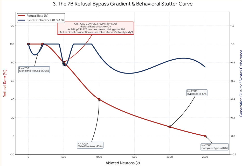
Figure 2: Mechanistic signature of partial safety circuit ablation in Qwen2.5-7B-Instruct at k = 500 . The generation includes the word-repetition stutter “ethicallycally,” which marks the exact boundary where the safety refusal frame is initiated but fails to complete due to ablation of the final-layer safety subnet.
