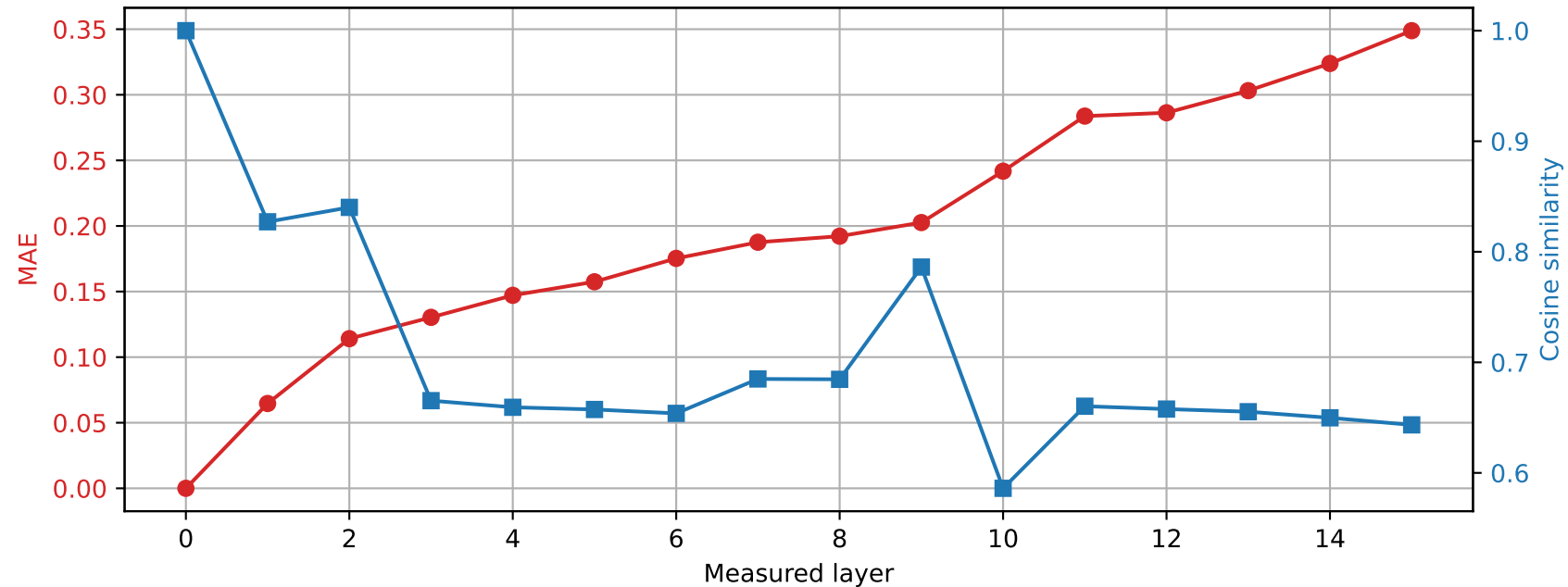
OLMo-1B-hf | Prompt 0 Spared layer 1 | Hybrid vs unquantized
