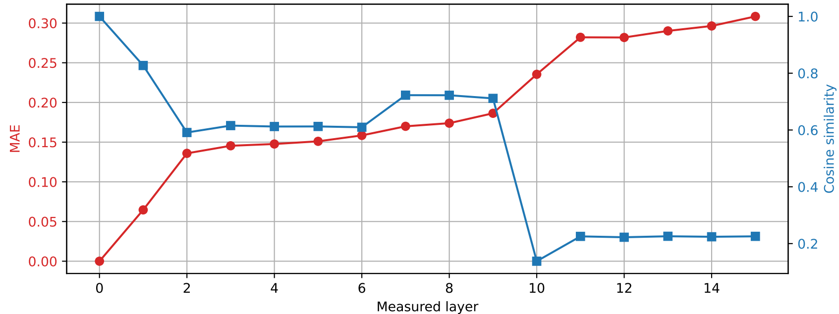
OLMo-1B-hf | Prompt 0 Spared layer 3 | Hybrid vs unquantized
