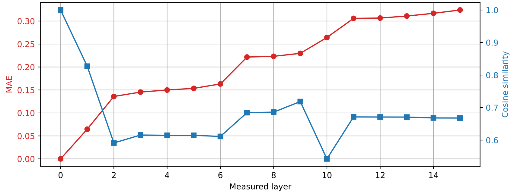
OLMo-1B-hf | Prompt 0 Spared layer 6 | Hybrid vs unquantized
