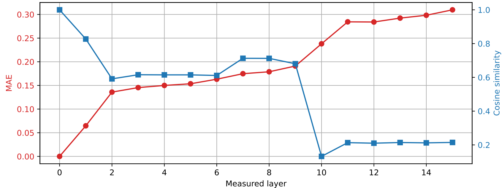
OLMo-1B-hf | Prompt 0 Spared layer 14 | Hybrid vs unquantized
