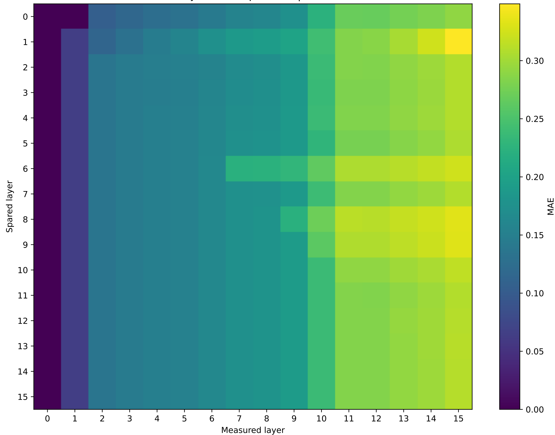
OLMo-1B-hf | Prompt 0 Hybrid vs unquantized | int4
