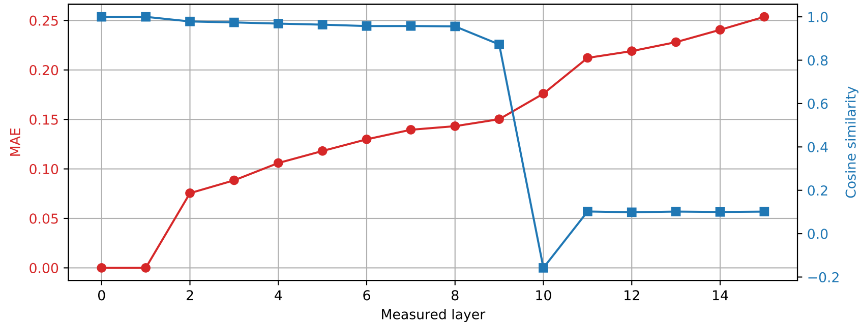
OLMo-1B-hf | Prompt 1 Spared layer 0 | Hybrid vs unquantized
