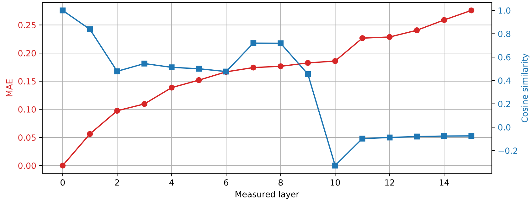
OLMo-1B-hf | Prompt 1 Spared layer 3 | Hybrid vs unquantized
