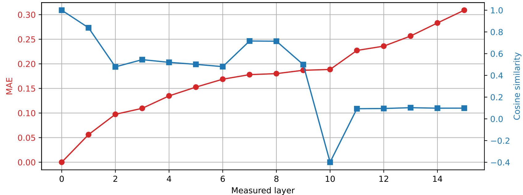
OLMo-1B-hf | Prompt 1 Spared layer 7 | Hybrid vs unquantized
