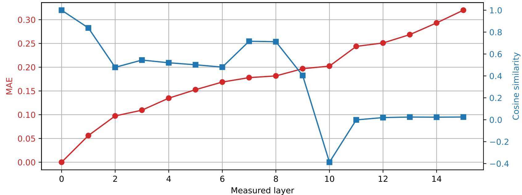
OLMo-1B-hf | Prompt 1 Spared layer 8 | Hybrid vs unquantized
