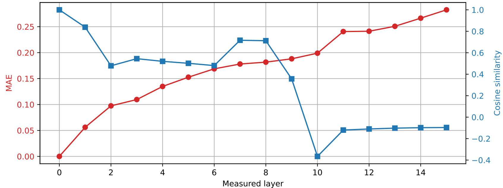
OLMo-1B-hf | Prompt 1 Spared layer 9 | Hybrid vs unquantized
