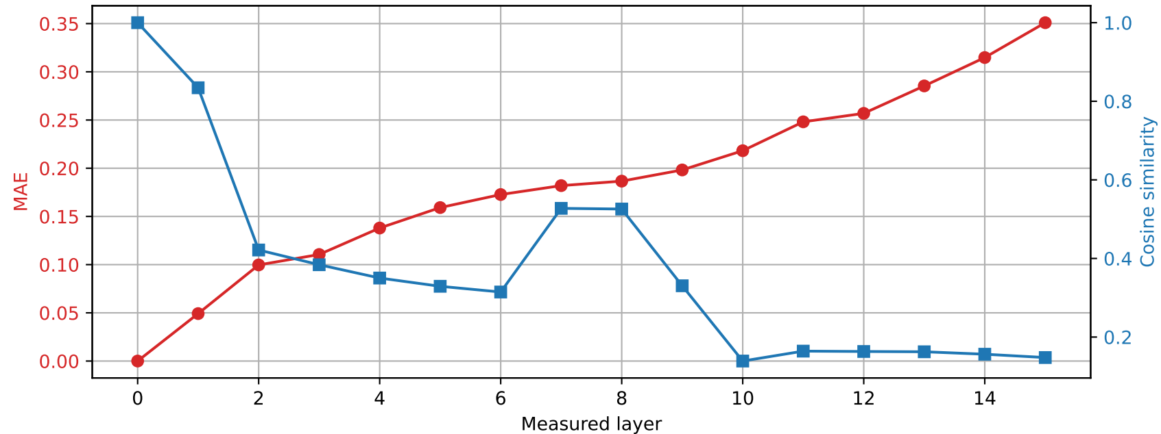
OLMo-1B-hf | Prompt 2 Spared layer 9 | Hybrid vs unquantized
