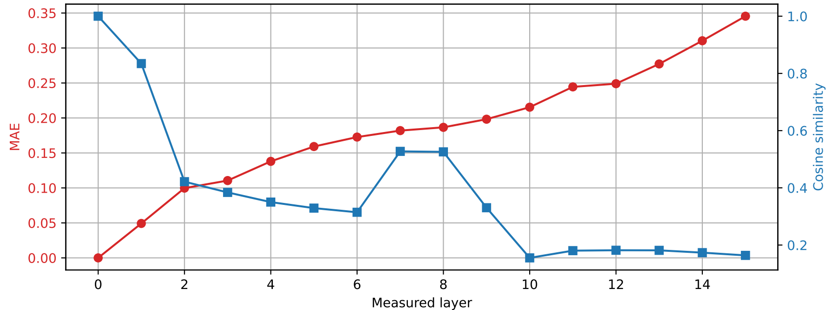
OLMo-1B-hf | Prompt 2 Spared layer 11 | Hybrid vs unquantized
