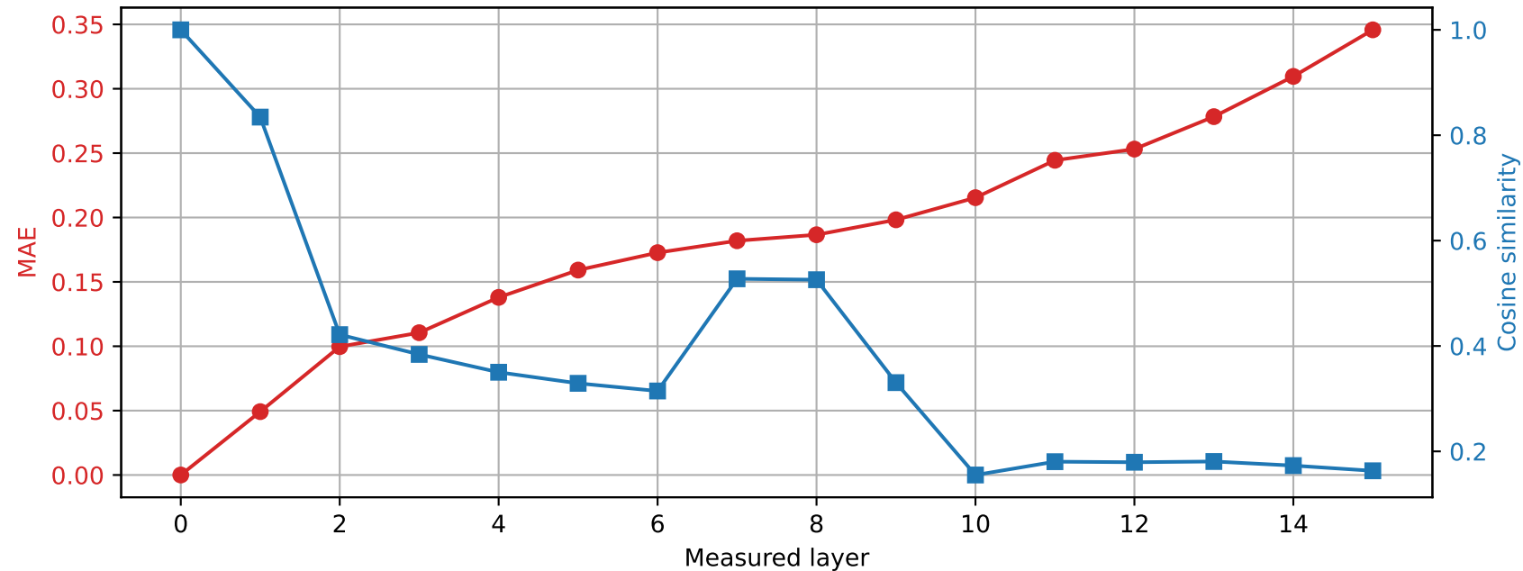
OLMo-1B-hf | Prompt 2 Spared layer 12 | Hybrid vs unquantized
