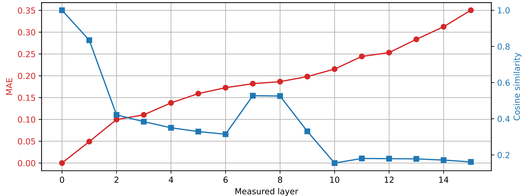
OLMo-1B-hf | Prompt 2 Spared layer 13 | Hybrid vs unquantized
