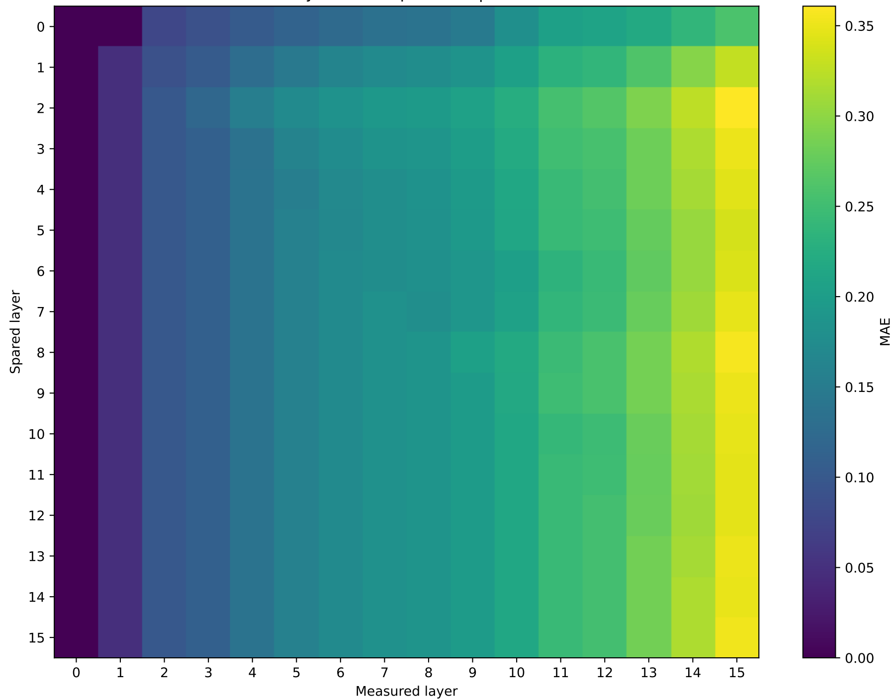
OLMo-1B-hf | Prompt 2 Hybrid vs unquantized | int4
