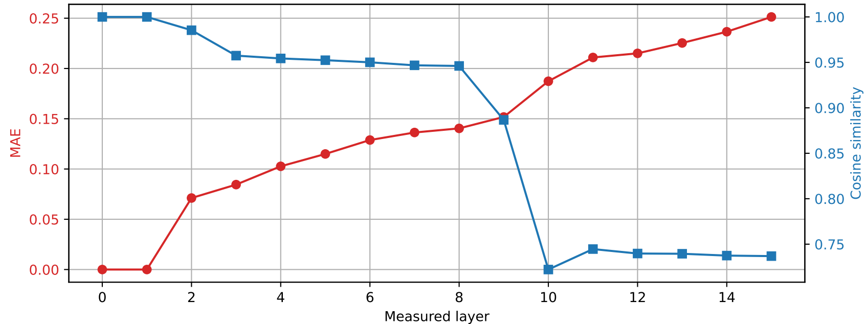
OLMo-1B-hf | Prompt 3 Spared layer 0 | Hybrid vs unquantized
