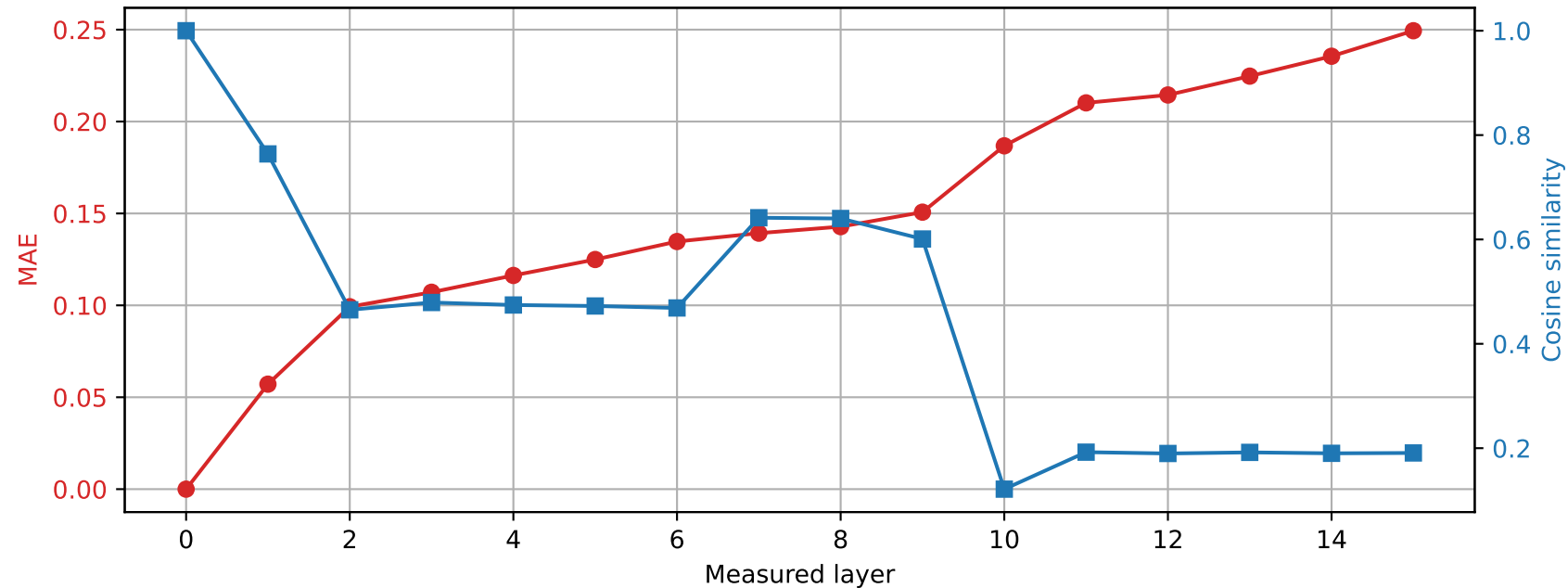
OLMo-1B-hf | Prompt 3 Spared layer 7 | Hybrid vs unquantized
