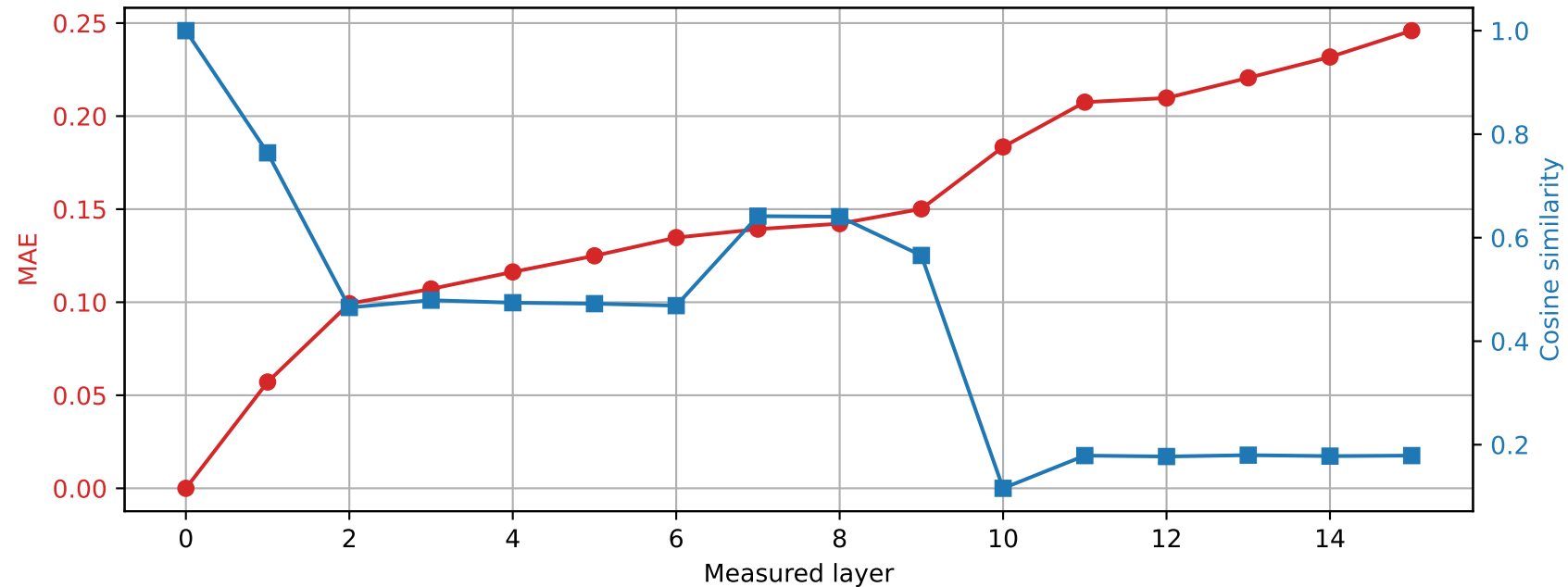
OLMo-1B-hf | Prompt 3 Spared layer 11 | Hybrid vs unquantized
