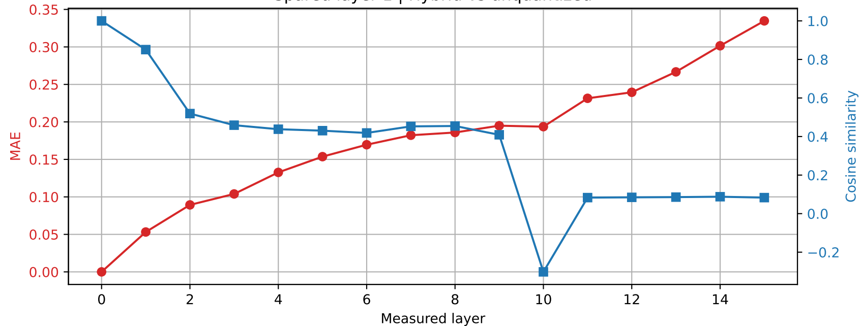
OLMo-1B-hf | Prompt 4 Spared layer 1 | Hybrid vs unquantized
