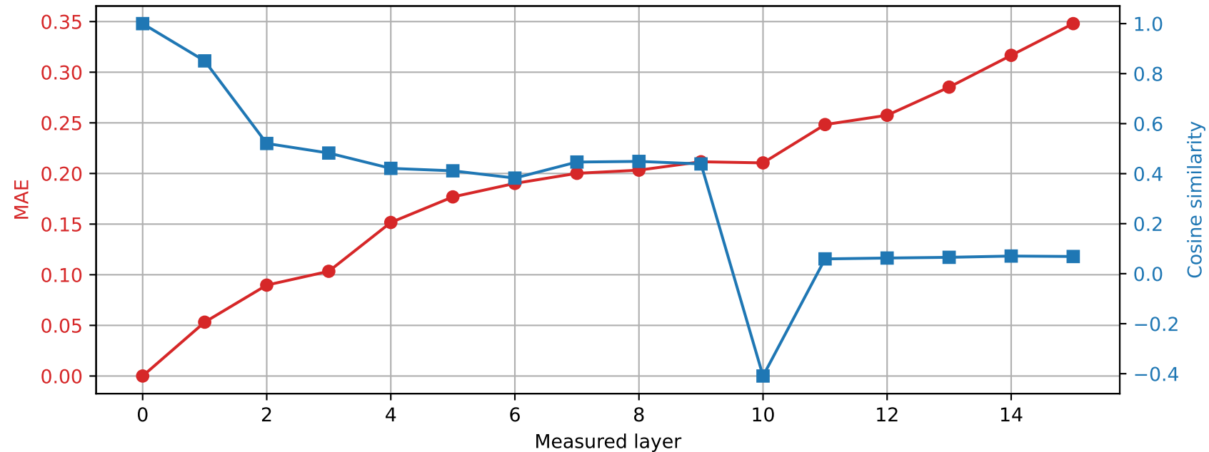
OLMo-1B-hf | Prompt 4 Spared layer 3 | Hybrid vs unquantized
