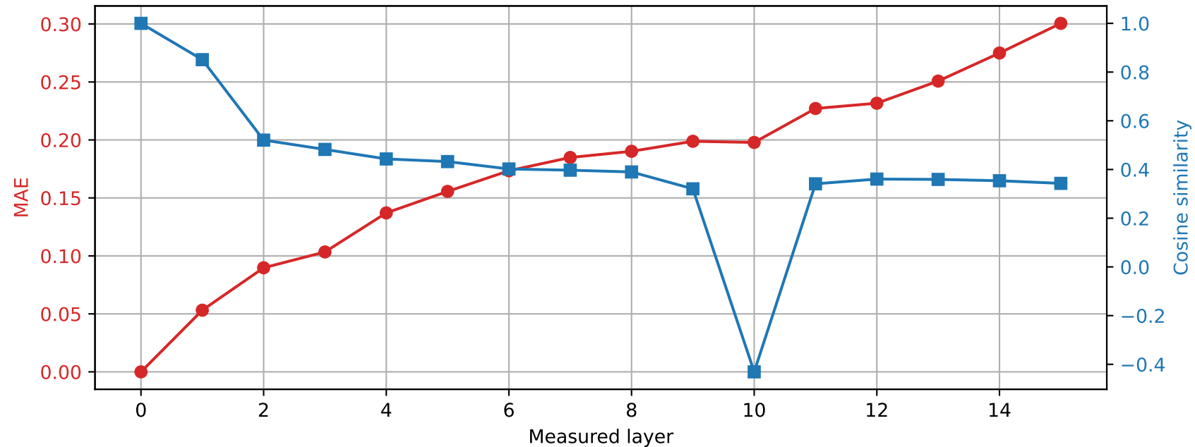
OLMo-1B-hf | Prompt 4 Spared layer 10 | Hybrid vs unquantized
