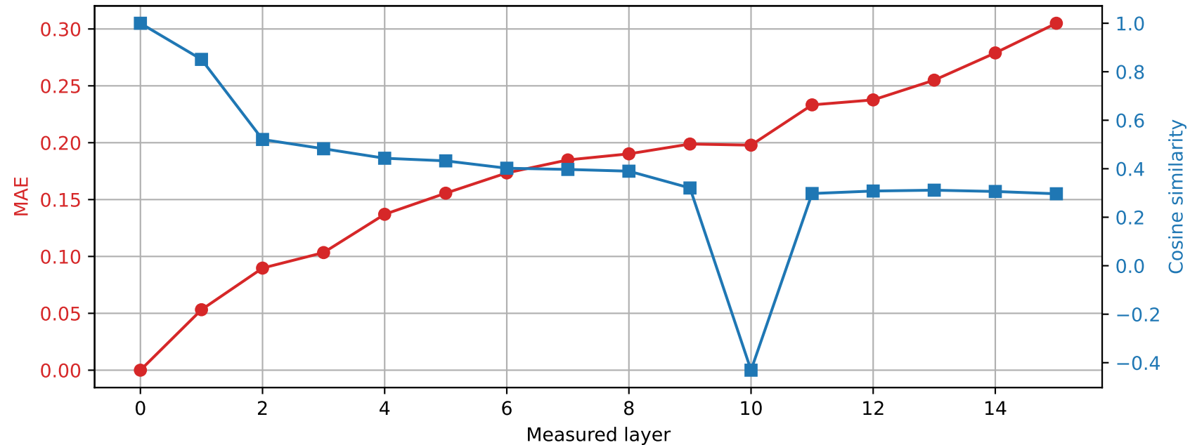
OLMo-1B-hf | Prompt 4 Spared layer 12 | Hybrid vs unquantized
