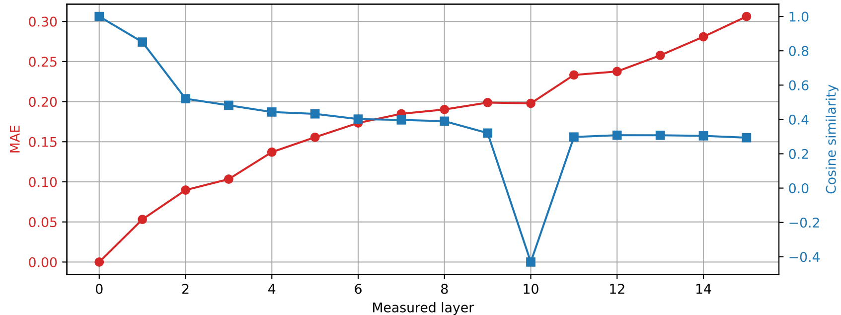
OLMo-1B-hf | Prompt 4 Spared layer 14 | Hybrid vs unquantized
