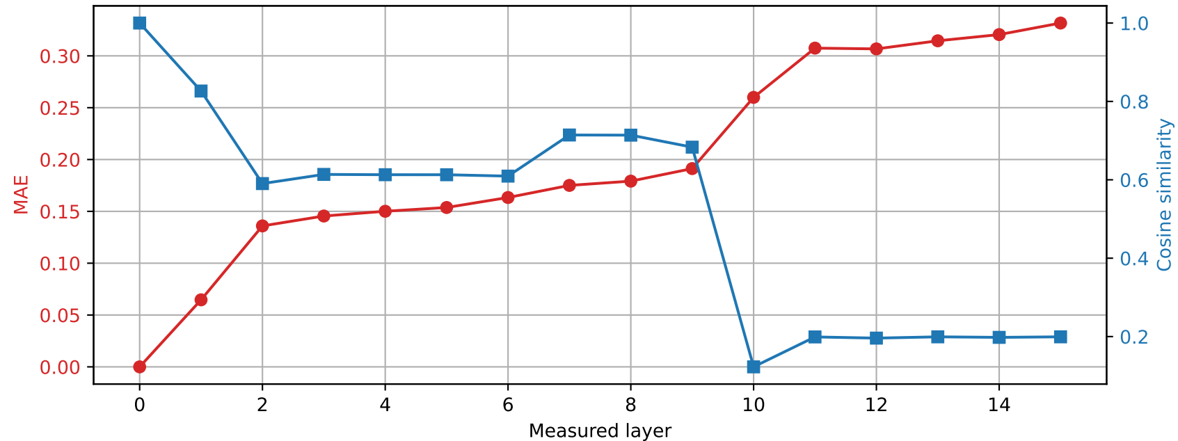
OLMo-1B-hf | Prompt 0 Spared layer 9 | Hybrid vs unquantized
