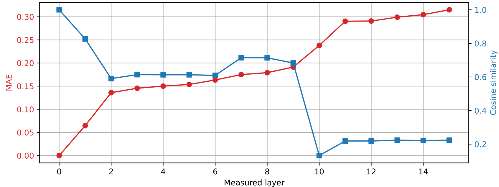
OLMo-1B-hf | Prompt 0 Spared layer 10 | Hybrid vs unquantized
