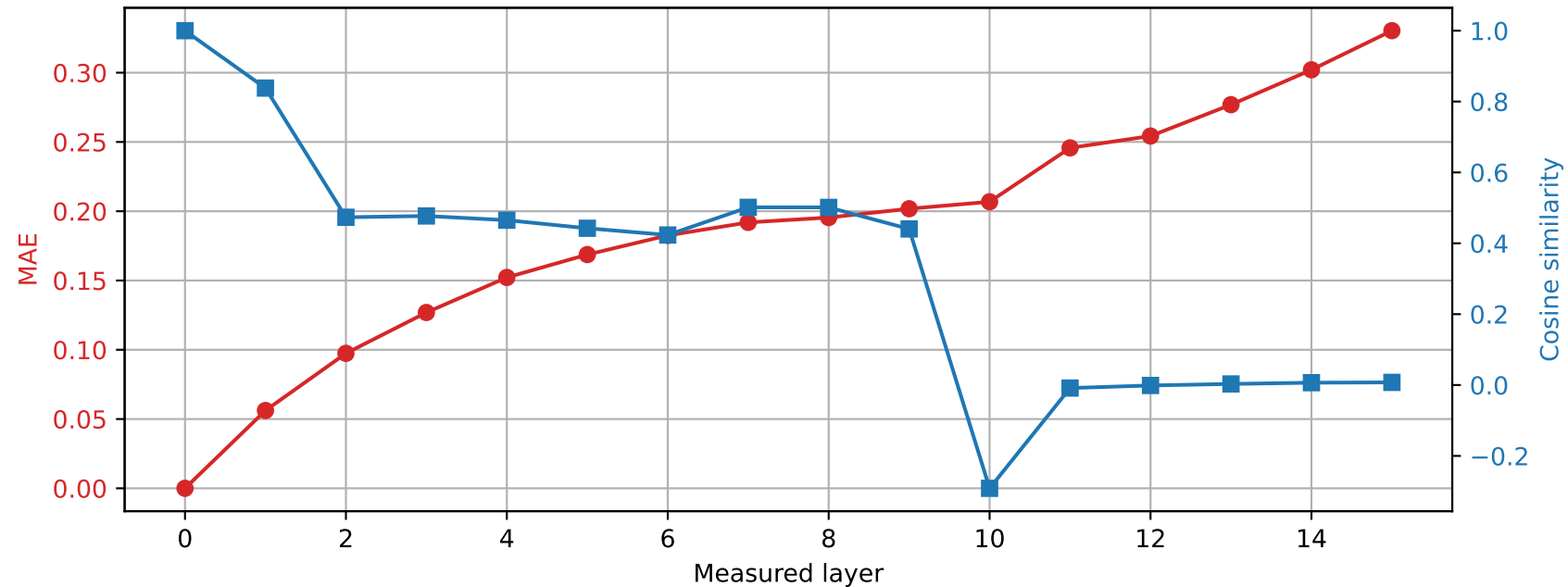
OLMo-1B-hf | Prompt 1 Spared layer 2 | Hybrid vs unquantized
