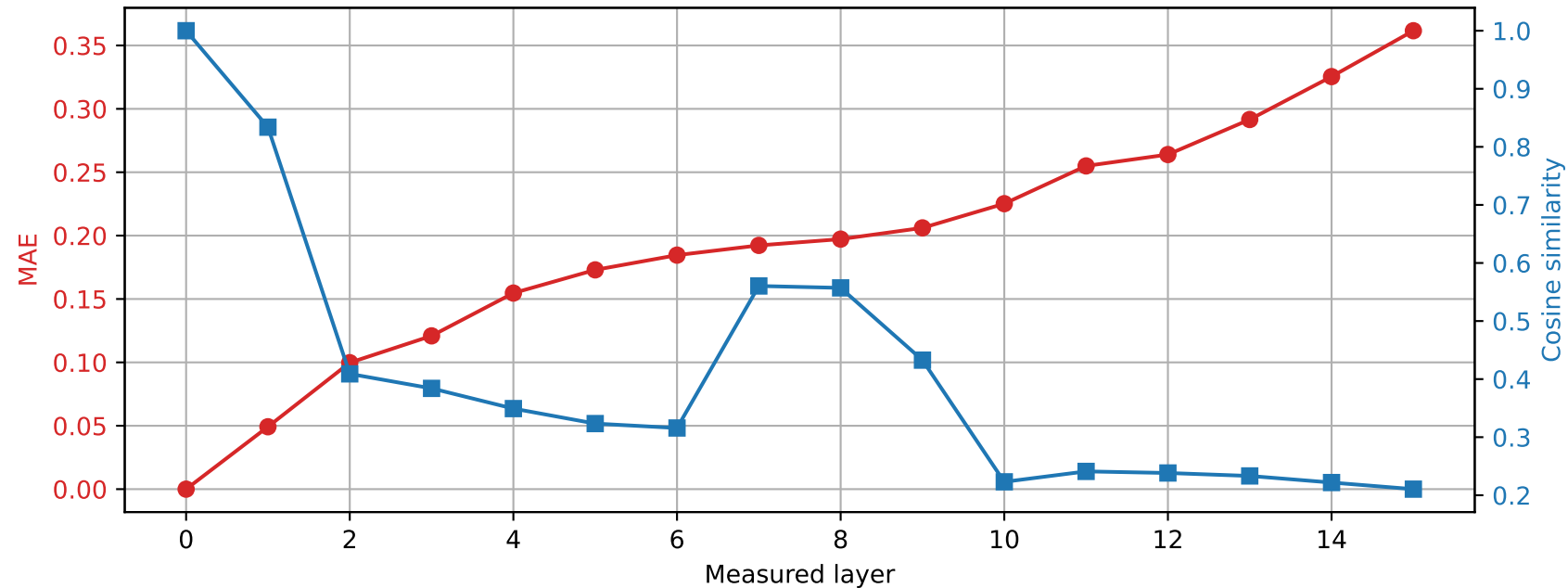
OLMo-1B-hf | Prompt 2 Spared layer 2 | Hybrid vs unquantized
