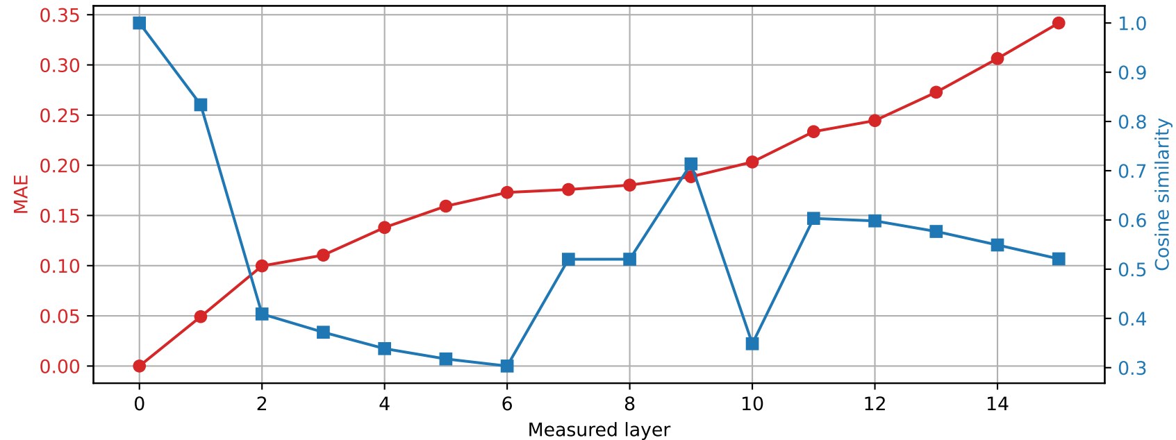
OLMo-1B-hf | Prompt 2 Spared layer 6 | Hybrid vs unquantized
