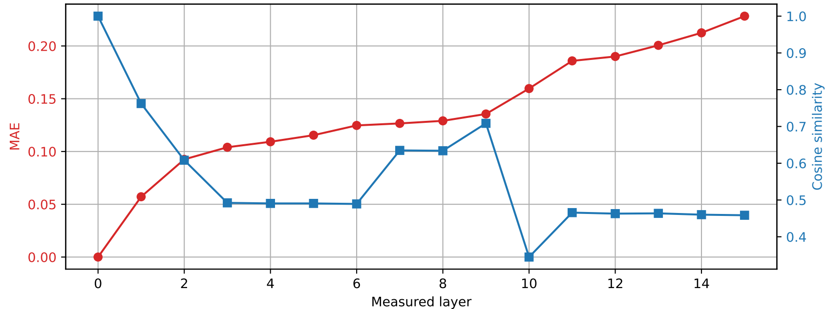
OLMo-1B-hf | Prompt 3 Spared layer 1 | Hybrid vs unquantized
