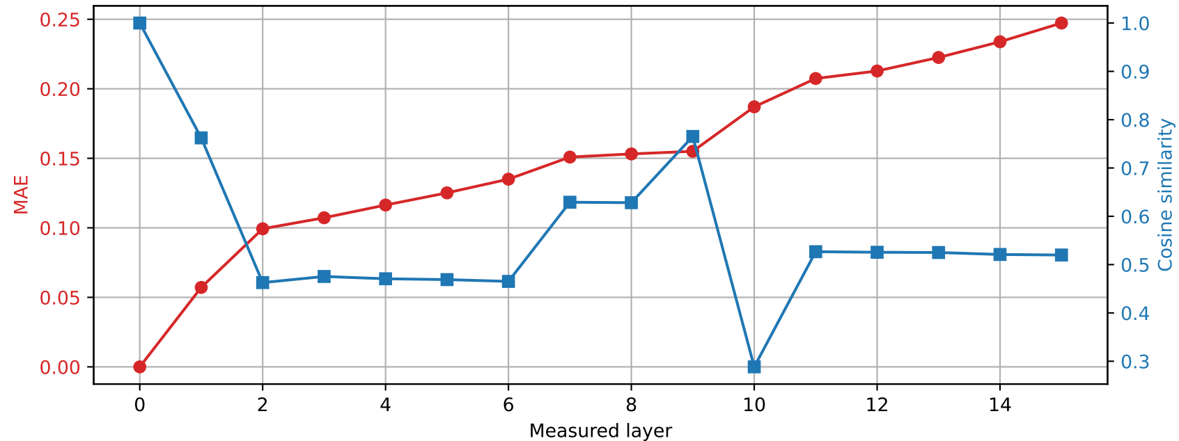
OLMo-1B-hf | Prompt 3 Spared layer 6 | Hybrid vs unquantized
