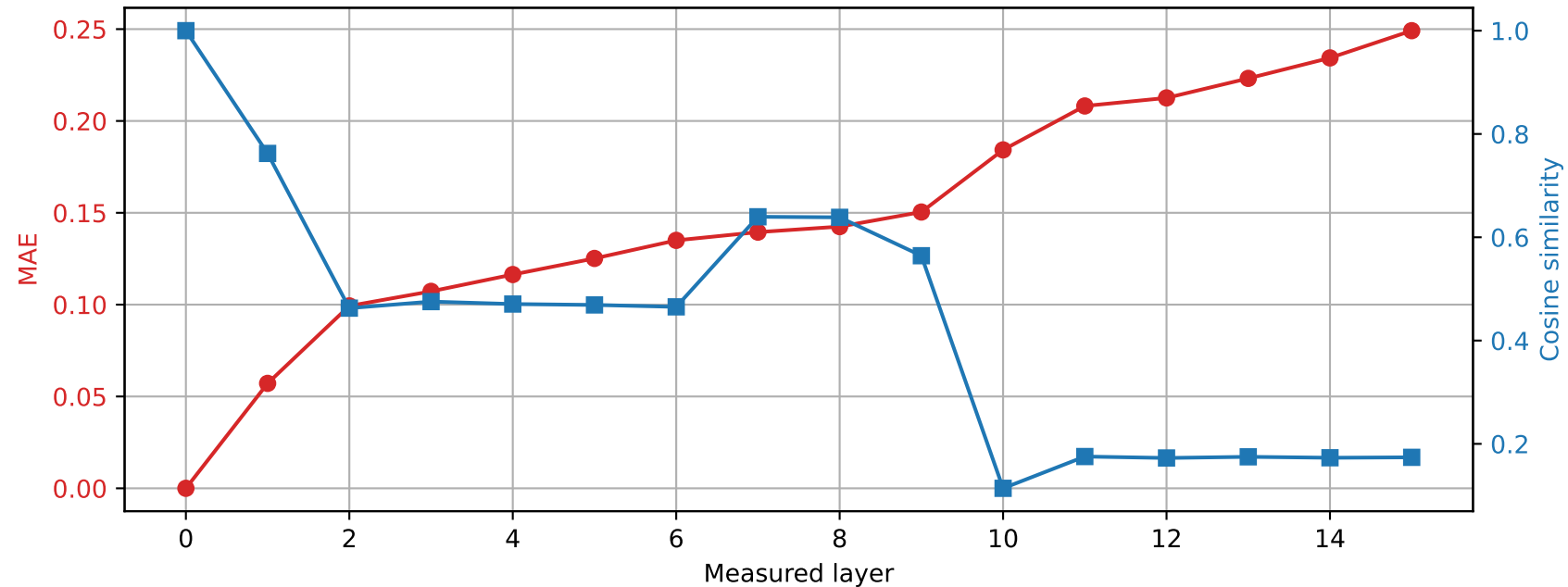
OLMo-1B-hf | Prompt 3 Spared layer 15 | Hybrid vs unquantized
