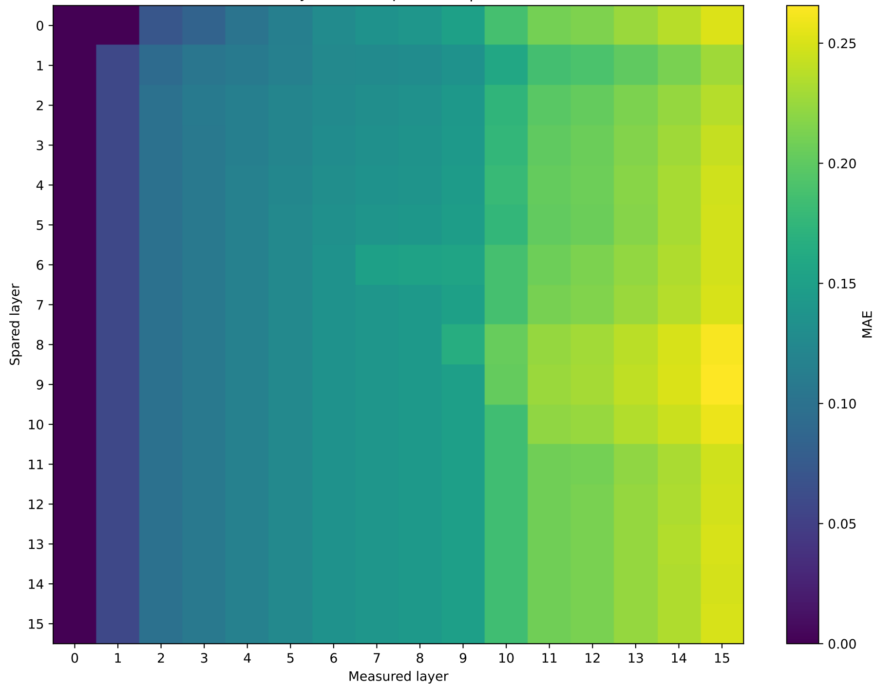
OLMo-1B-hf | Prompt 3 Hybrid vs unquantized | int4
