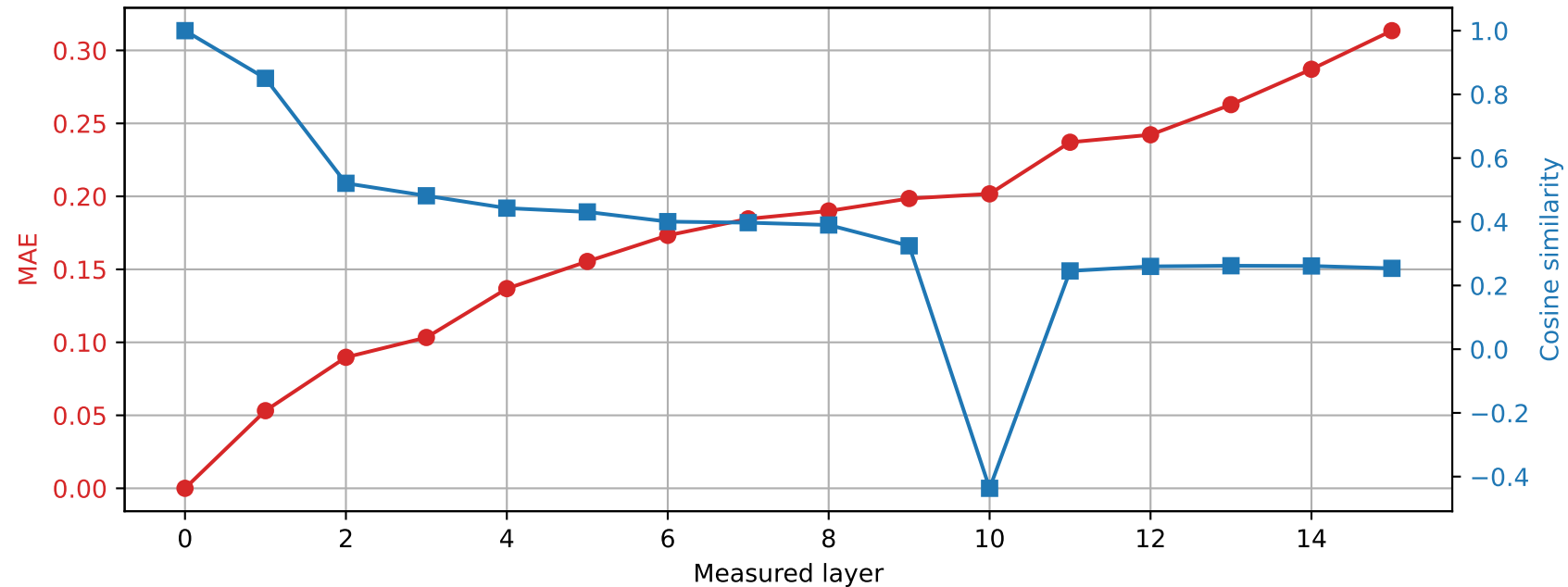
OLMo-1B-hf | Prompt 4 Spared layer 9 | Hybrid vs unquantized
