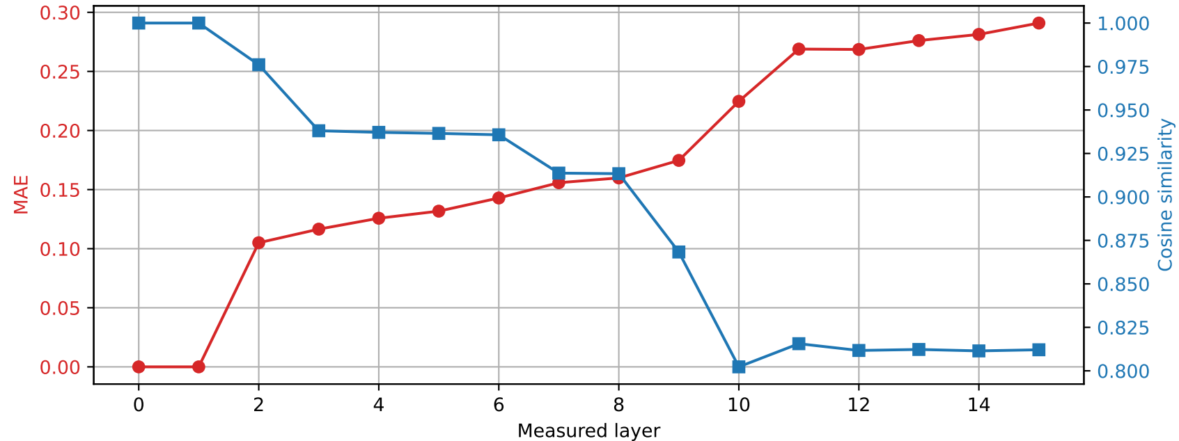
OLMo-1B-hf | Prompt 0 Spared layer 0 | Hybrid vs unquantized
