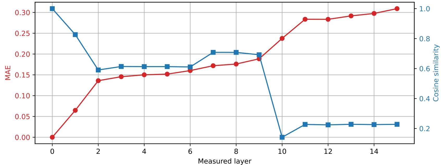
OLMo-1B-hf | Prompt 0 Spared layer 4 | Hybrid vs unquantized
