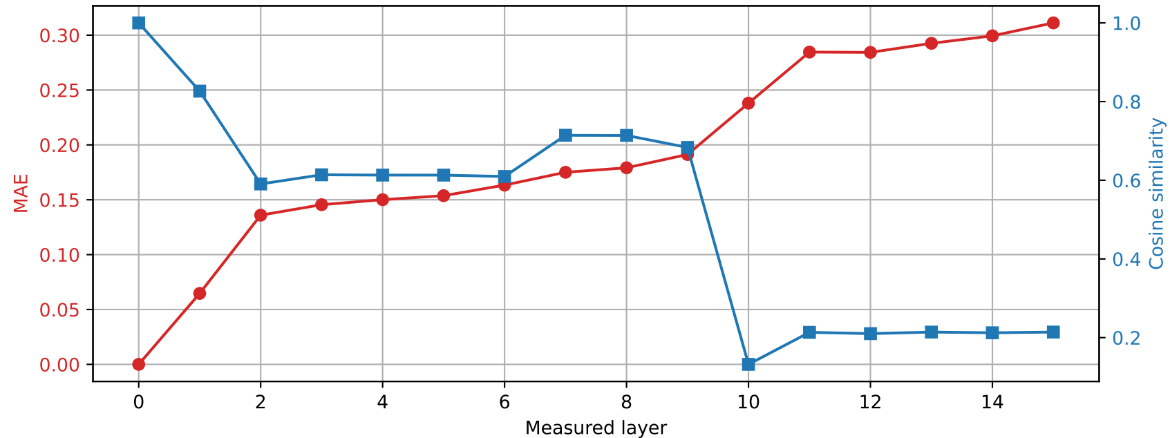
OLMo-1B-hf | Prompt 0 Spared layer 13 | Hybrid vs unquantized
