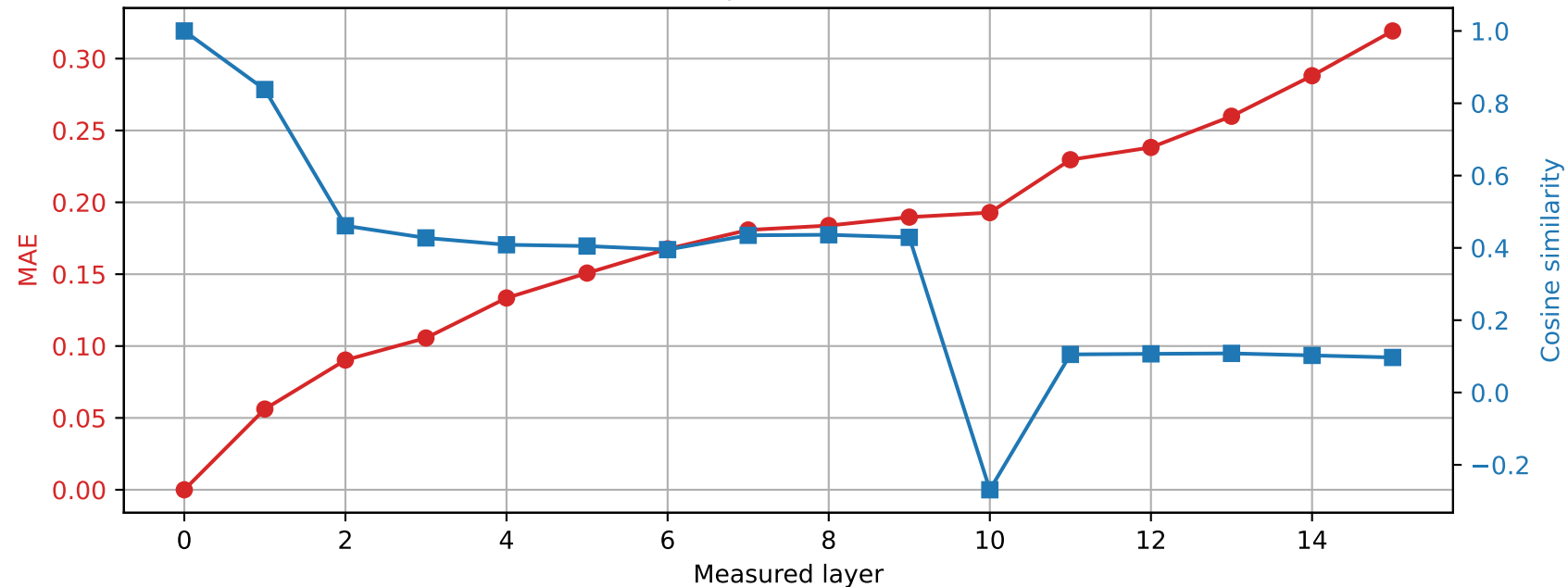
OLMo-1B-hf | Prompt 1 Spared layer 1 | Hybrid vs unquantized
