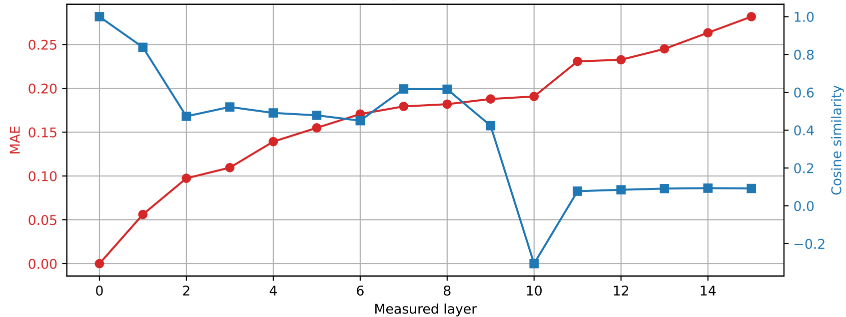
OLMo-1B-hf | Prompt 1 Spared layer 3 | Hybrid vs unquantized
