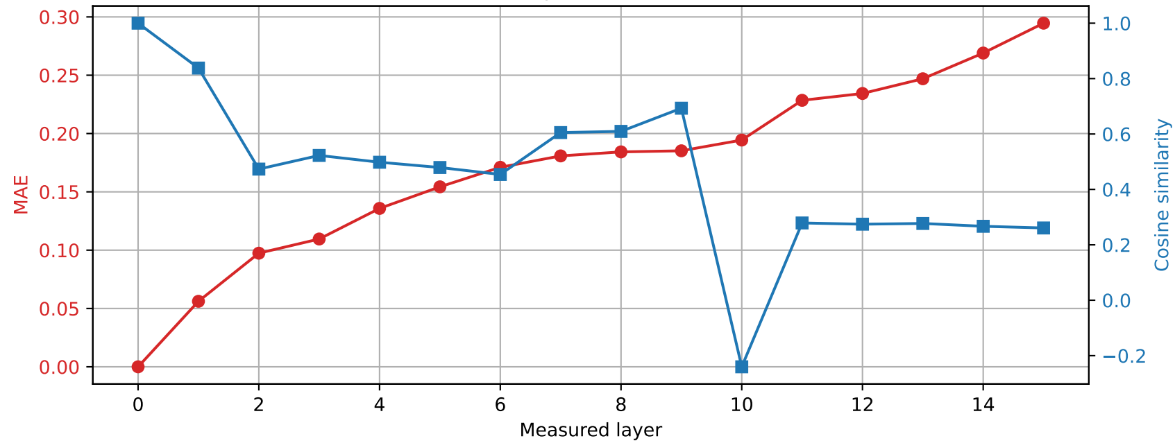
OLMo-1B-hf | Prompt 1 Spared layer 6 | Hybrid vs unquantized
