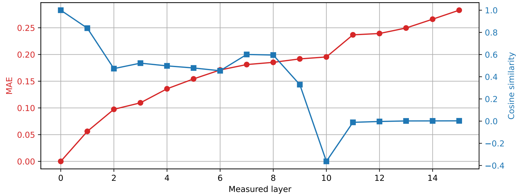
OLMo-1B-hf | Prompt 1 Spared layer 11 | Hybrid vs unquantized
