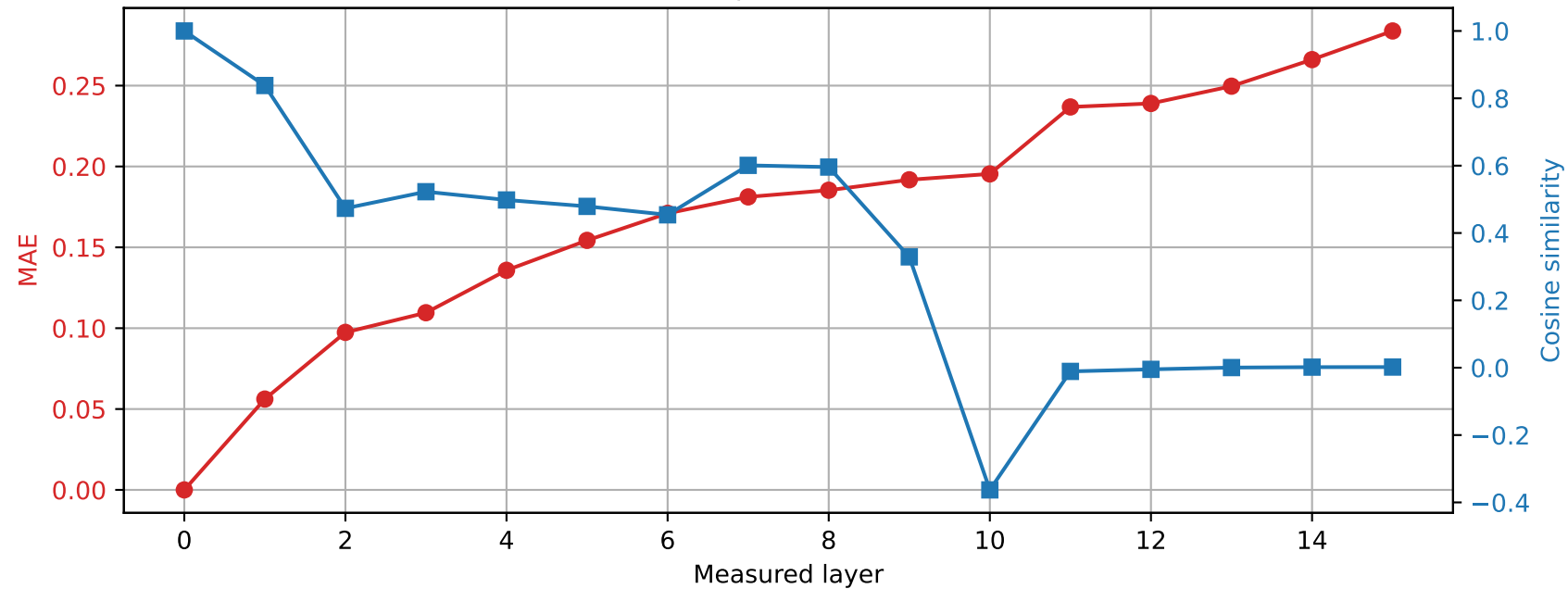
OLMo-1B-hf | Prompt 1 Spared layer 13 | Hybrid vs unquantized
