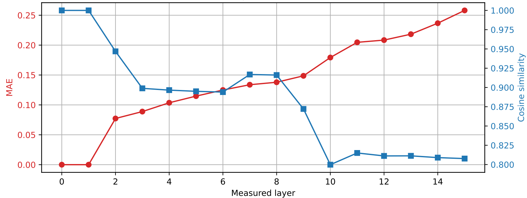
OLMo-1B-hf | Prompt 2 Spared layer 0 | Hybrid vs unquantized
