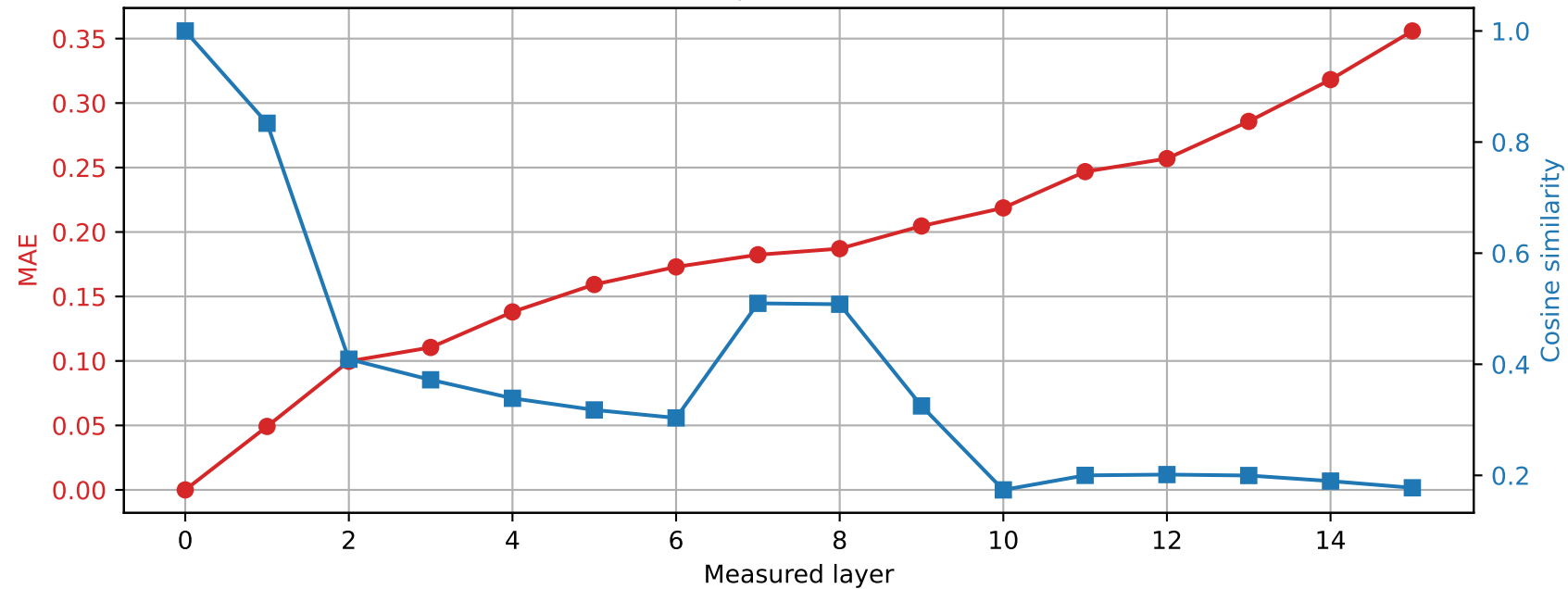
OLMo-1B-hf | Prompt 2 Spared layer 8 | Hybrid vs unquantized
