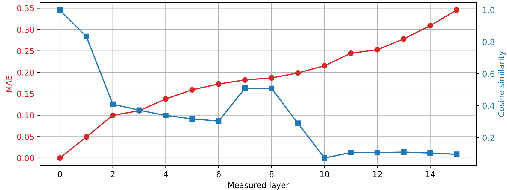
OLMo-1B-hf | Prompt 2 Spared layer 12 | Hybrid vs unquantized
